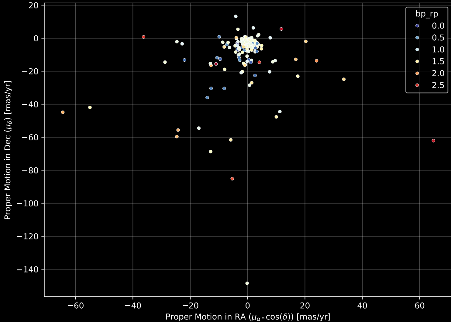
APOGEE DR17 Field: [180+18] Proper Motion Diagram (n= 186)
