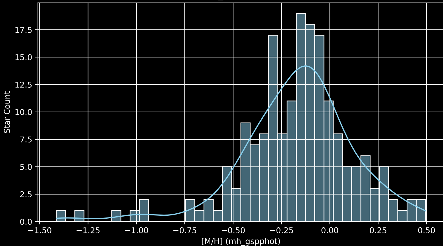
APOGEE DR17 Field: [180+18 [M/H] (mh_gspphot) (n= 184)
