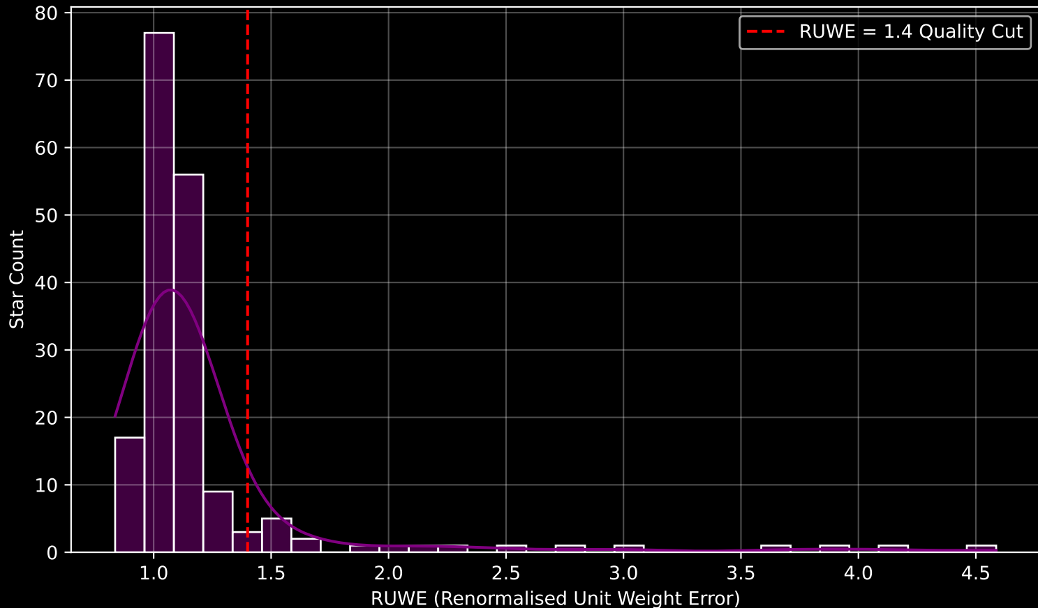
GAPOGEE DR17 Field [180+18] RUWE Distribution (n= 180)
