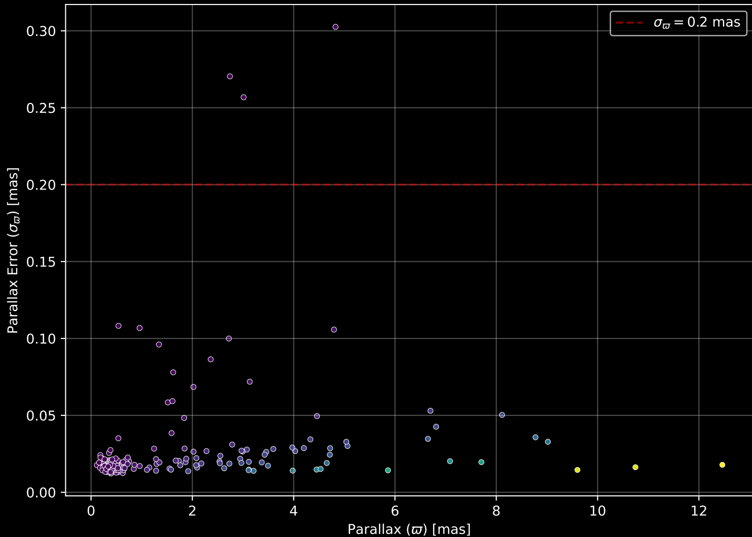
APOGEE DR17 Field: [180+18] Parallax Quality (n= 186)
