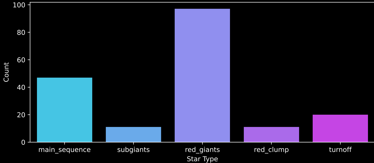
APOGEE DR17 Field: [180+18] Count plot of Star Type
